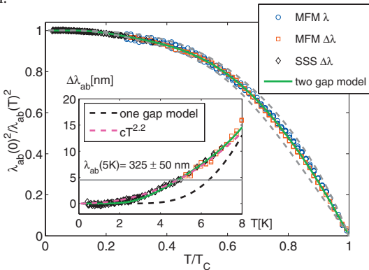
FIG. 2. (Color) Normalized superfluid density \rho_s(T)/\rho_s(0) \equiv \lambda_{ab}(0)^2/\lambda_{ab}(T)^2 vs T . We determine \Delta\lambda_{ab}(T) by MFM (squares) and by SSS (diamonds) from measuring the change in the diamagnetic response at fixed height. These values are offset to match the absolute value of \lambda_{ab}(T) obtained by fitting the MFM data to the truncated cone model (circles). The green solid line shows a fit of the two-band s -wave model discussed in the main text ( \Delta_1=2.6T_c , \Delta_2=0.8T_c , x=0.88 , and a=1.4 ). The width of the dashed band reflects the uncertainty in \lambda_{ab}(0) . Inset: \Delta\lambda_{ab} vs T at low T . Black dashed line: one-gap s -wave model with a=1.5 and \Delta_0=1.95T_c . Magenta dashed line: \Delta\lambda_{ab}(T)=cT^{2.2} ( c=0.14 nm/ \text{K}^{2.2} ).
