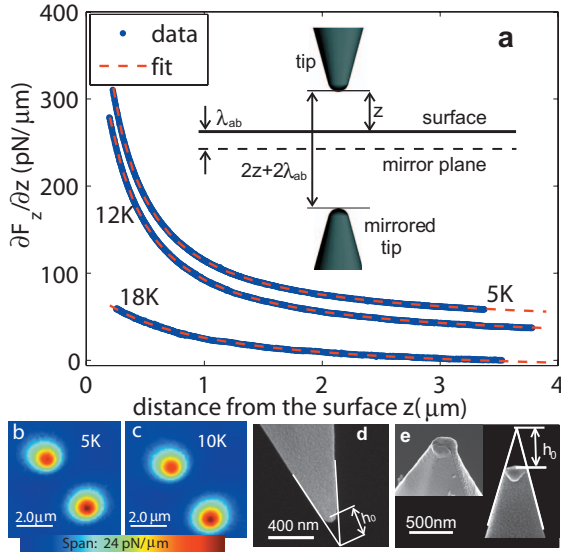
FIG. 1. (Color) Technique to measure \lambda and \Delta\lambda by MFM from (a) Meissner repulsion and [(b) and (c)] vortex imaging. (a) z dependence of \partial F_z/\partial z (blue symbols) at T=5, 12 , and 18 K and the fit to the truncated cone model (red dashed line). (Inset) Sketch to illustrate that the tip-superconductor interaction in the Meissner state can be approximated by the interaction between the tip and its image mirrored through a plane (dashed line) \lambda_{ab} below the surface of the superconductor (solid line) when z \gg \lambda_{ab} . Comparing the curves provides \Delta\lambda_{ab} independently of the tip model. Fits give \lambda_{ab}(T) at T=5, 12, 18 K to be 0.33, 0.37, 1.10 \mu\text{m} . [(b) and (c)] Images of two vortices ( z=400 nm) at (b) 5 and (c) 10 K. The similar shapes and amplitudes of the images show that both the spatial variation and the temperature-induced change in \lambda_{ab} are small. [(d) and (e)] Scanning electron microscopy images of the tip (d) before and (e) after the measurements. An accidental crash during the measurement changes the truncation distance h_0 from (d) 300 \pm 30 nm to (e) 400 \pm 20 nm. Despite the crash, \partial F_z/\partial z curves taken before and after the crash give the same \lambda_{ab}(5 K) to within 10 nm.
