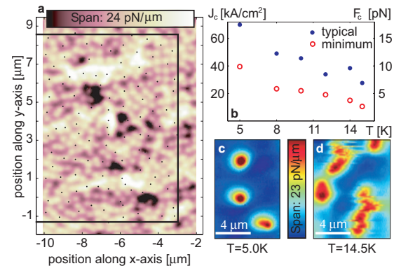
FIG. 4. (Color) Inhomogeneous vortex pinning. (a) Image of vortices at T=5 K, z=80 nm, and B=9.5 mT, overlaid by the vortex positions (dots) in Fig. 3(a) and the boundary of that scan (black frame). The vortex configuration is highly disordered. Vortices avoid the same regions in both scans, taken days apart and many thermal cycles apart. (b) Local critical current (left ordinate) and the depinning force (right ordinate) vs T . The comparison of minimum and typical values implies inhomogeneous pinning. (c) Image of vortices at T=5 K, z=120 nm showing that F_{\min} only moves the vortex at the bottom. (d) Image of moving vortices at T=14.5 K, z=430 nm showing that F_{\text{typ}} allows us to drag all vortices a distance of several microns.
