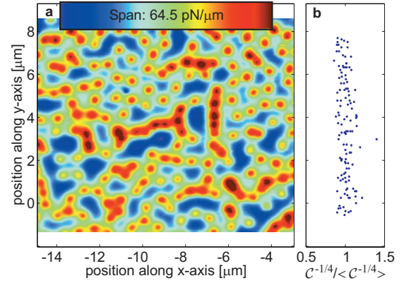
FIG. 3. (Color) Spatial uniformity of \lambda_{ab} from vortex imaging at 5 K. (a) Image of vortices at T=5 K, z=125 nm, and a vortex density giving 3.5 mT. (b) The normalized length scale associated with each vortex peak in (a) C^{-1/4}/\langle C^{-1/4} \rangle ( \langle \rangle denotes the mean). We find C^{-1/4}=250(1 \pm 0.08) nm (70% confidence interval).
